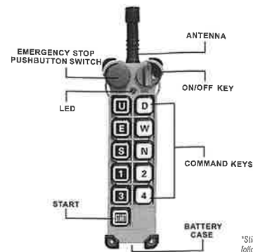
Fig.6: Model 4S, 6S, 8S, 10S
